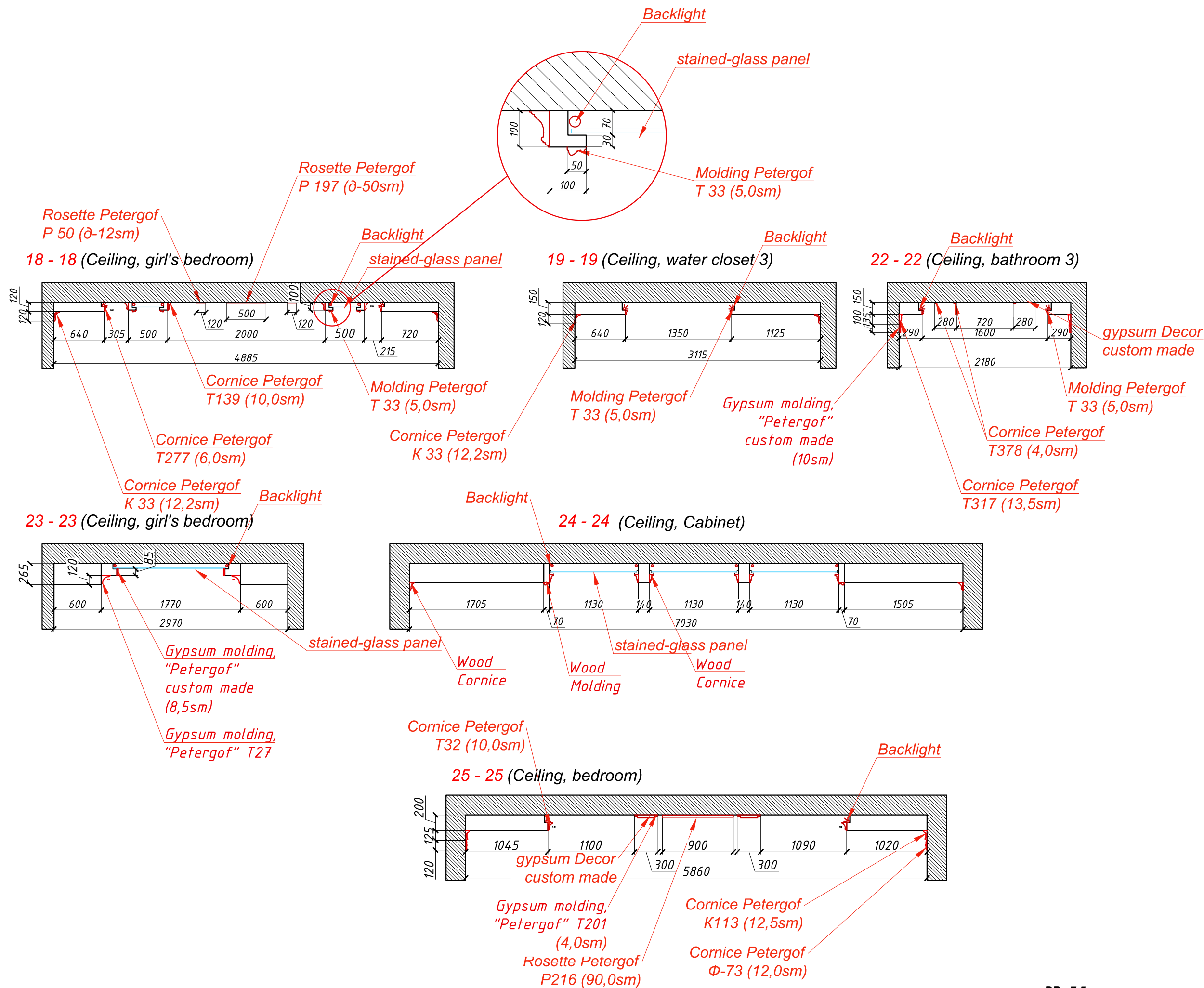
DP - 7.5 Ceiling section scheme
